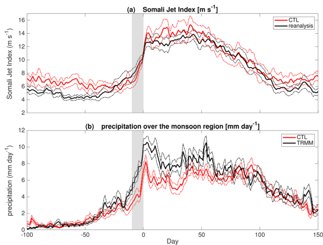
Figure 1. Composite evolution of (a) the Somali jet index and (b) averaged precipitation over the South Asian monsoon region in the control simulation (red) and reanalysis data or satellite observation (black). The dashed curves denote 95% confidence intervals. The day of onset is shifted to Day 0. The gray shading marks the period from Day -10 to Day 0. CTL = control run; TRMM = Tropical Rainfall Measuring Mission.
