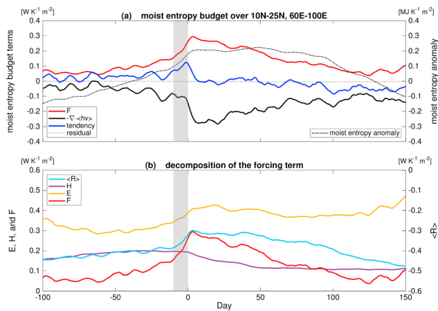
Figure 3. Composite evolution of column-integrated moist entropy budget averaged over 10–25°N; 60°E to 100°E in the control run. (a) The red, black, blue, and dashed curves denote the source term, the export by large-scale advection, the temporal tendency term, and the residual of the moist budget, respectively, and correspond to the left y axis. The dash-dotted curve denotes anomalous column-integrated moist entropy and corresponds to the right y axis. (b) The light blue curve denotes the contribution from radiative heating and corresponds to the right y axis. The purple, yellow, and red curves denote the sensible heat flux, the latent heat flux, and the sum of the source terms, respectively, and correspond to the left y axis.
