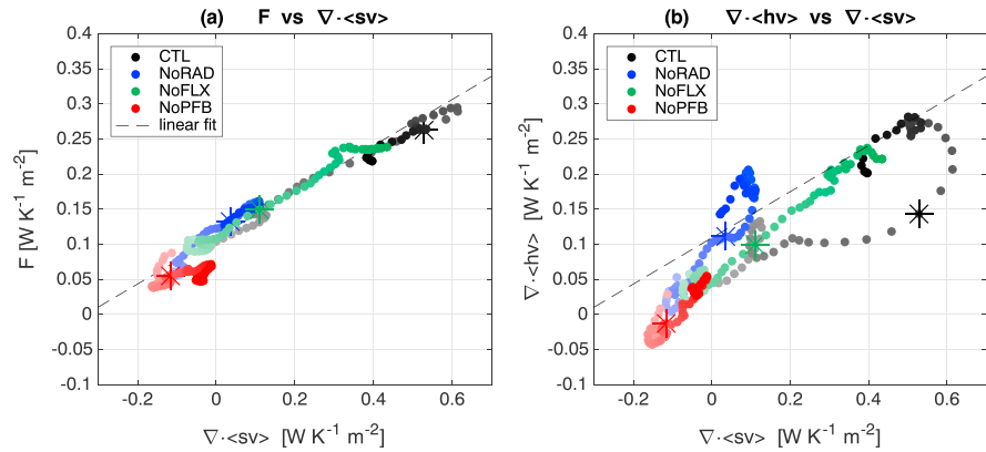
Figure 5. (a) Scatterplots of the sum of the source terms of column-integrated moist entropy against the divergence of column-integrated dry entropy. Each marker corresponds to 1 day from Day –30 to Day 30 with respect to the date of monsoon onset in CTL (denoted by the stars), and lighter colors indicate earlier dates. (b) The same as (a) but for the divergence of column-integrated moist entropy against the divergence of column-integrated dry entropy.
