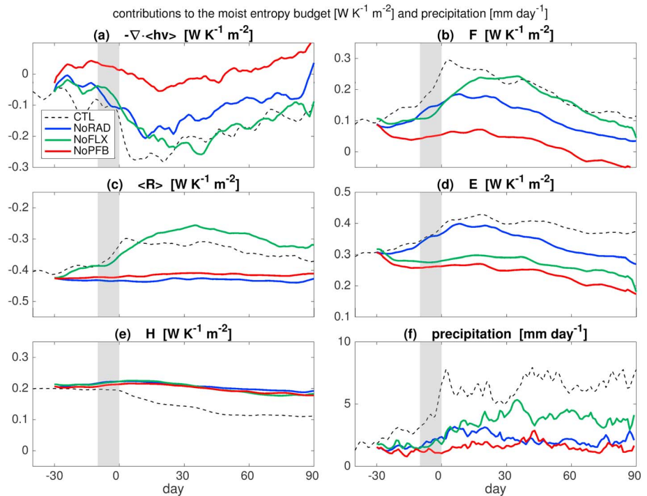
Figure 4. Composite evolution of column-integrated moist entropy budget terms (a–e) and precipitation (f) averaged over 10–25°N; 60°N to 100°E in the numerical simulations. The dashed, blue, green, and red curves denote the CTL, NoRAD, NoFLX, and NoPFB, respectively.
